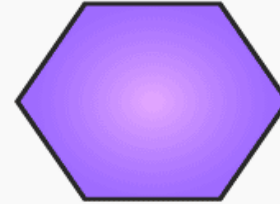
Hexagon
