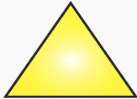
Triangle
