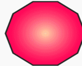
Decagon
