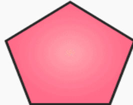
Pentagon
