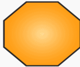
Octagon
