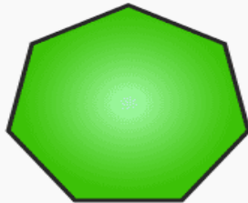
Heptagon
