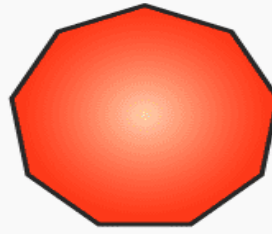
Nonagon
